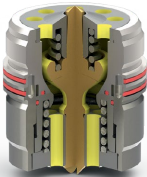
Engaged valve
