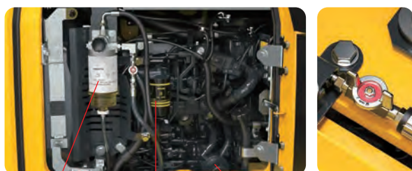
Fuel pre-filter (With water separator) High efficiency fuel filter Engine oil filter Fuel drain valve
