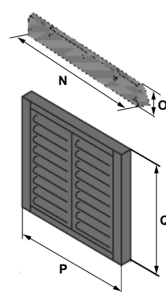
Right duct
