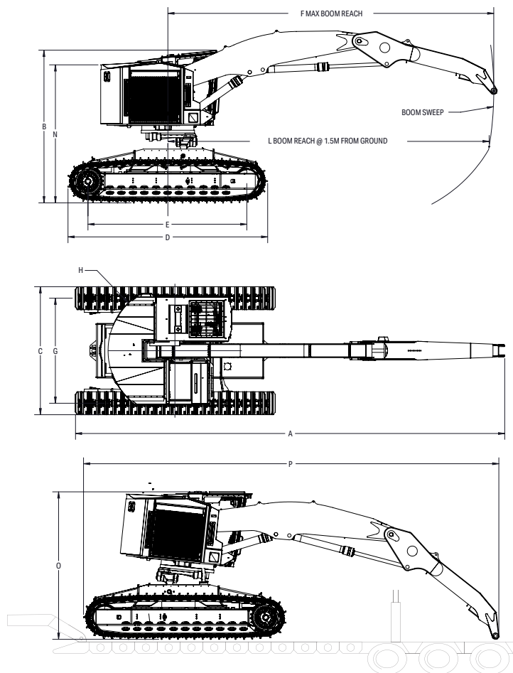
Transport dimensions: See C, O and P
